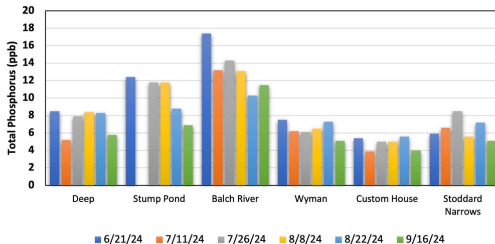
Figure 10. Balch Pond- 2024 Bi-weekly
