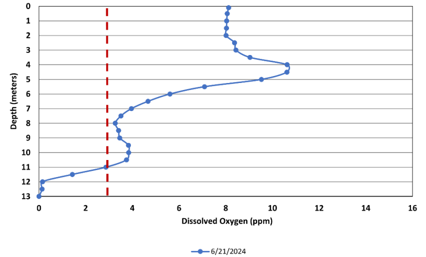
Figure 7. Balch Pond - Deep Site Dissolved Oxygen Profiles (June 21, 2024)
