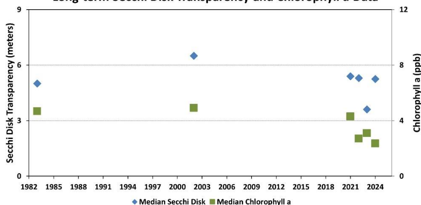
Figure 4. Balch Pond- Deep Site (1983-2024) Long-term Secchi Disk Transparency and Chlorophyll a Data
