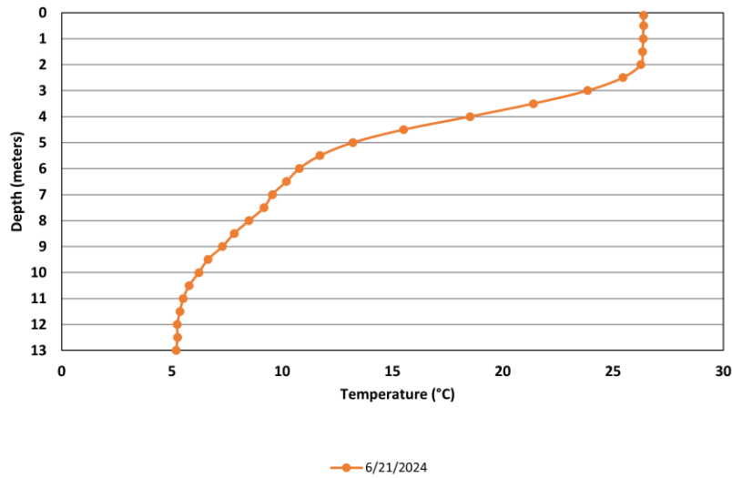
Figure 6. Balch Pond - Deep Site Temperature Profiles (June 21, 2024)
