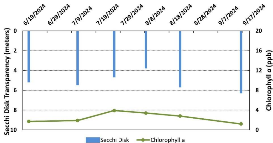
Figure 2. Balch Pond (2024 Seasonal Data) Secchi Disk Transparency and Chlorophyll a Data
