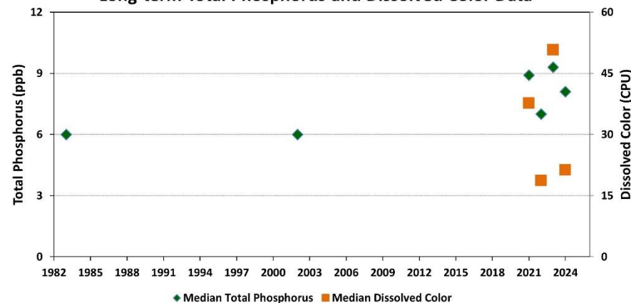
Figure 5. Balch Pond - Deep Site (1983-2024) Long-term Total Phosphorus and Dissolved Color Data
