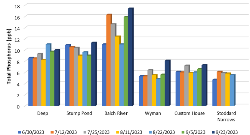
Figure 9. Balch Pond - 2023 Bi-weekly Total Phosphorus Inter-site Comparison
