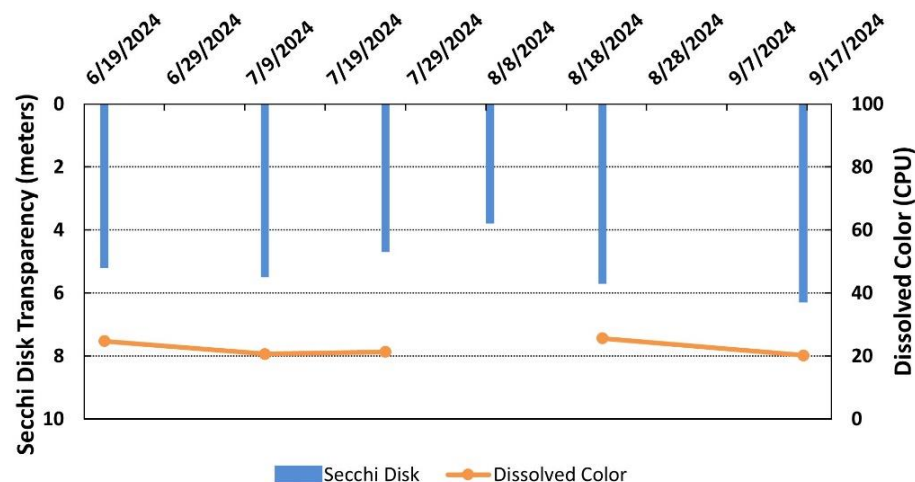
Figure 3. Balch Pond (2024 Seasonal Data) Secchi Disk Transparency and Dissolved Color Data
