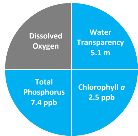
Figure 1. Balch Pond Water Quality (2024)
